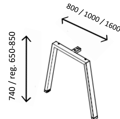
Noga trapez (A)
